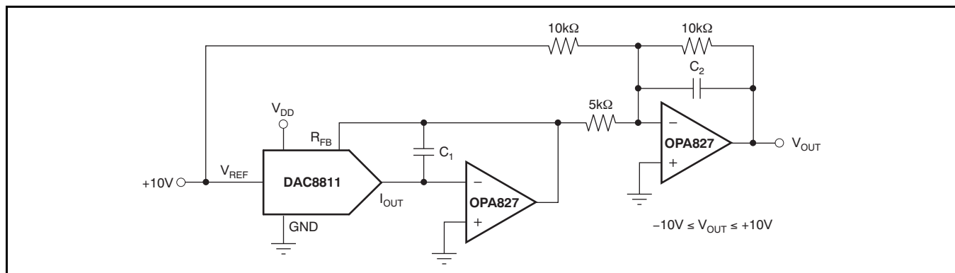
Figure 49. I/V Converter
